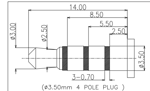
(ø3.50mm 4 POLE PLUG )
