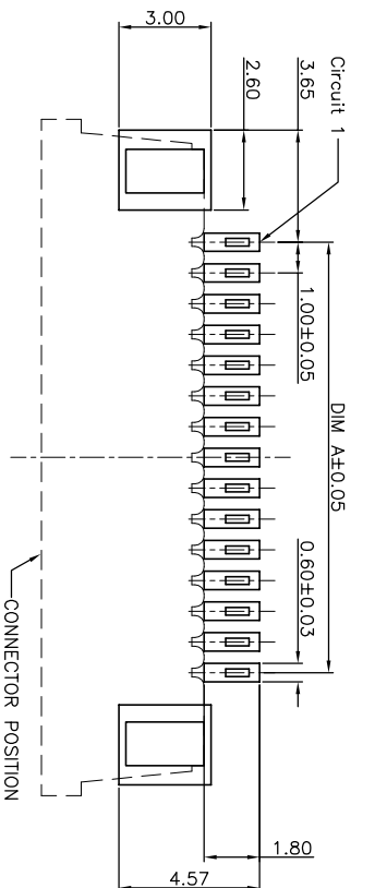
RECOMMENDED P.C.B. PATTERN LAYOUT
